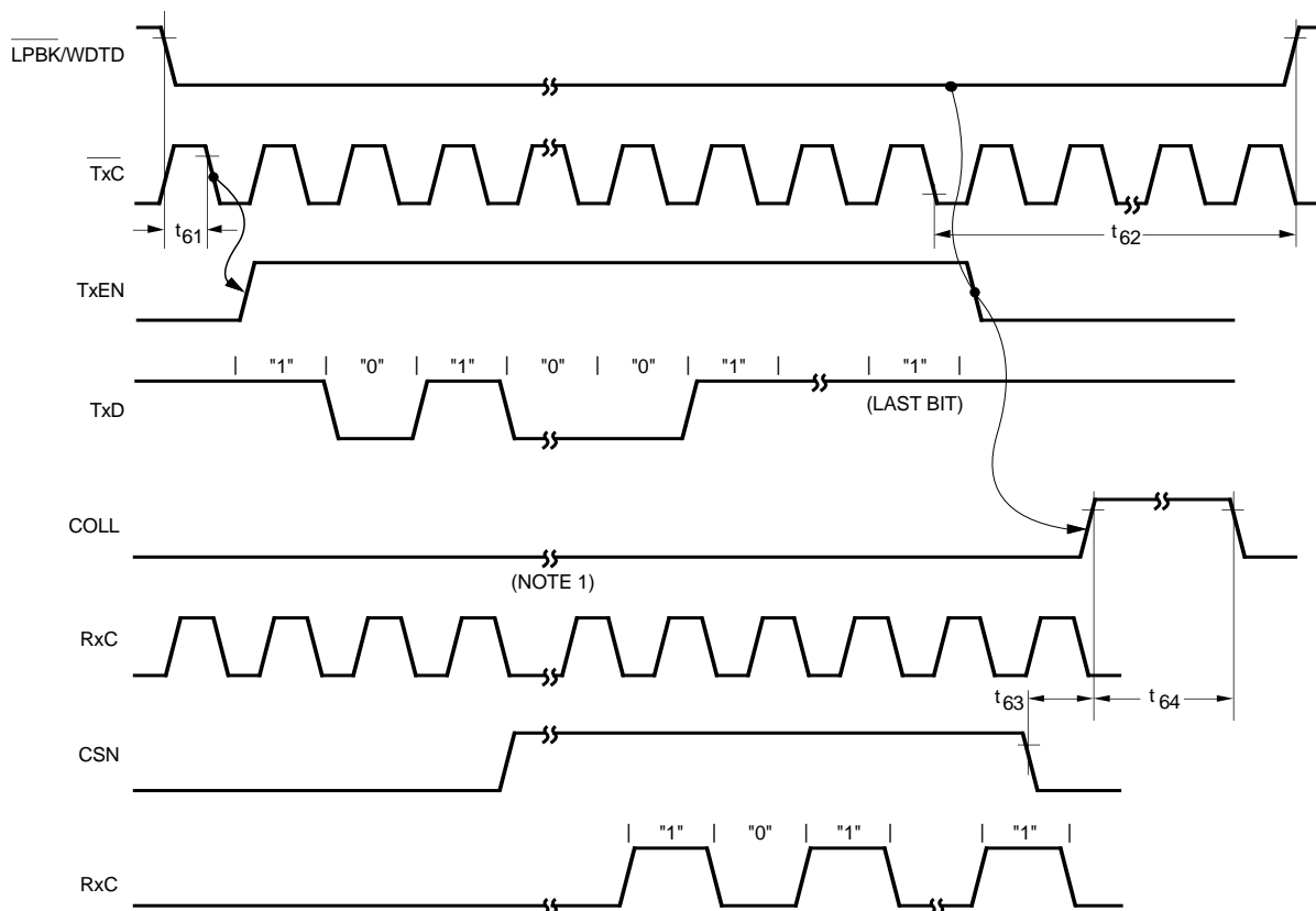
Figure 12. Loopback Timing
