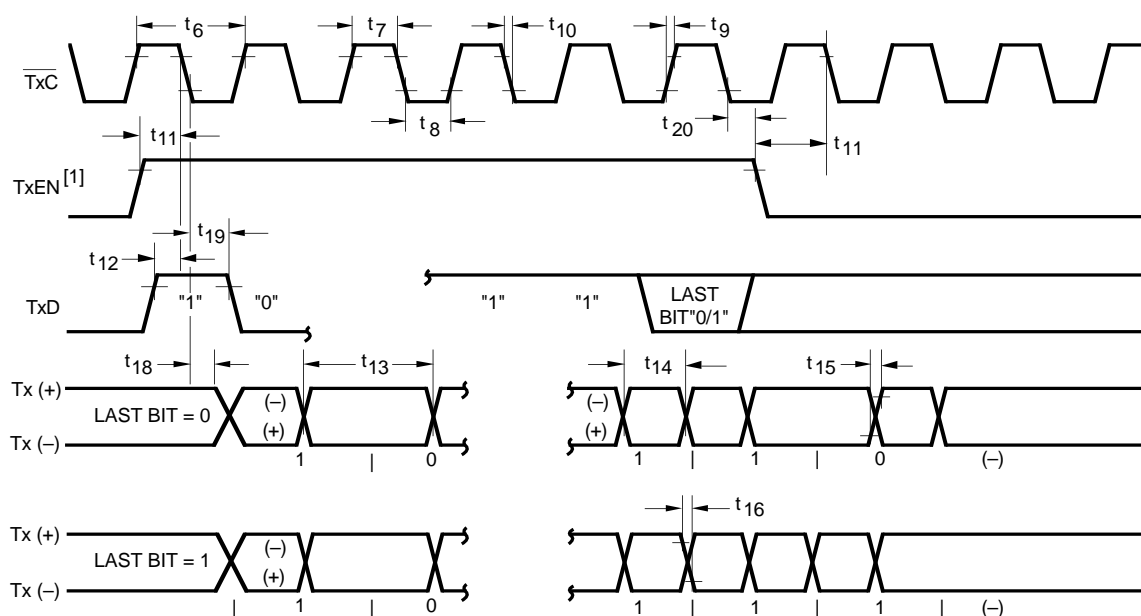
Figure 8. Transmit Timing
