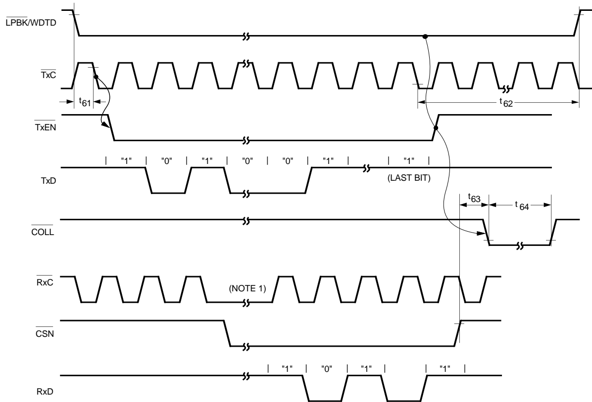
Figure 13. Loopback Timing —(Cont.)
