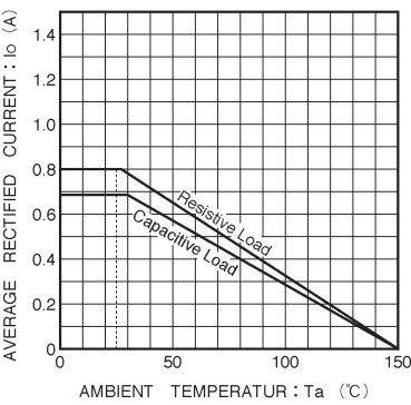
Fig. 3 Derating curve
