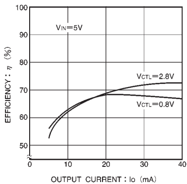
Fig. 3 Efficiency
