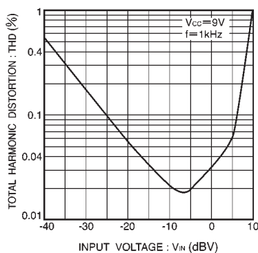
Fig. 4 Total harmonic distortion vs. input voltage
