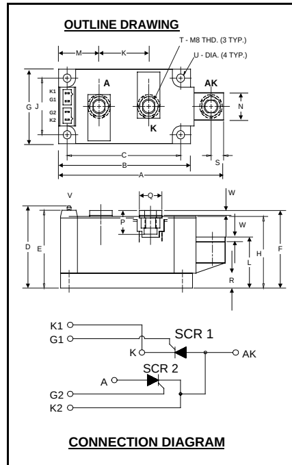
ND43_25 Dual SCR Isolated POW-R-BLOK™ Module 250 Amperes/1800 Volts
