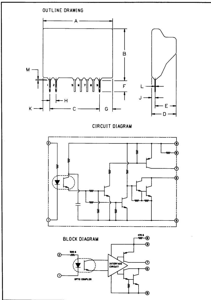
Outline Drawing
