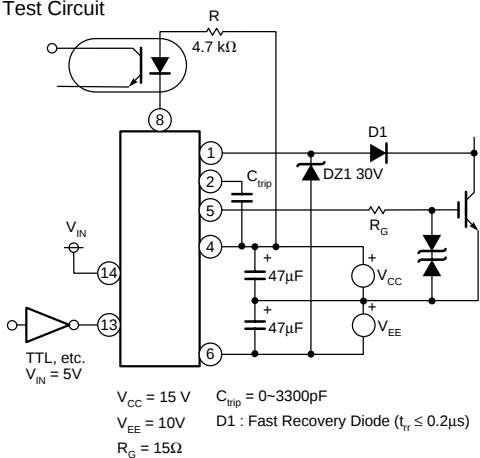
Test Circuit
