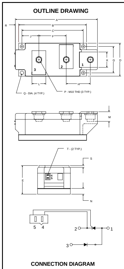
LD42__50 Dual SCR/Diode Pow-R-Blok™ Module 500 Amperes/ 600 – 1600 Volts
