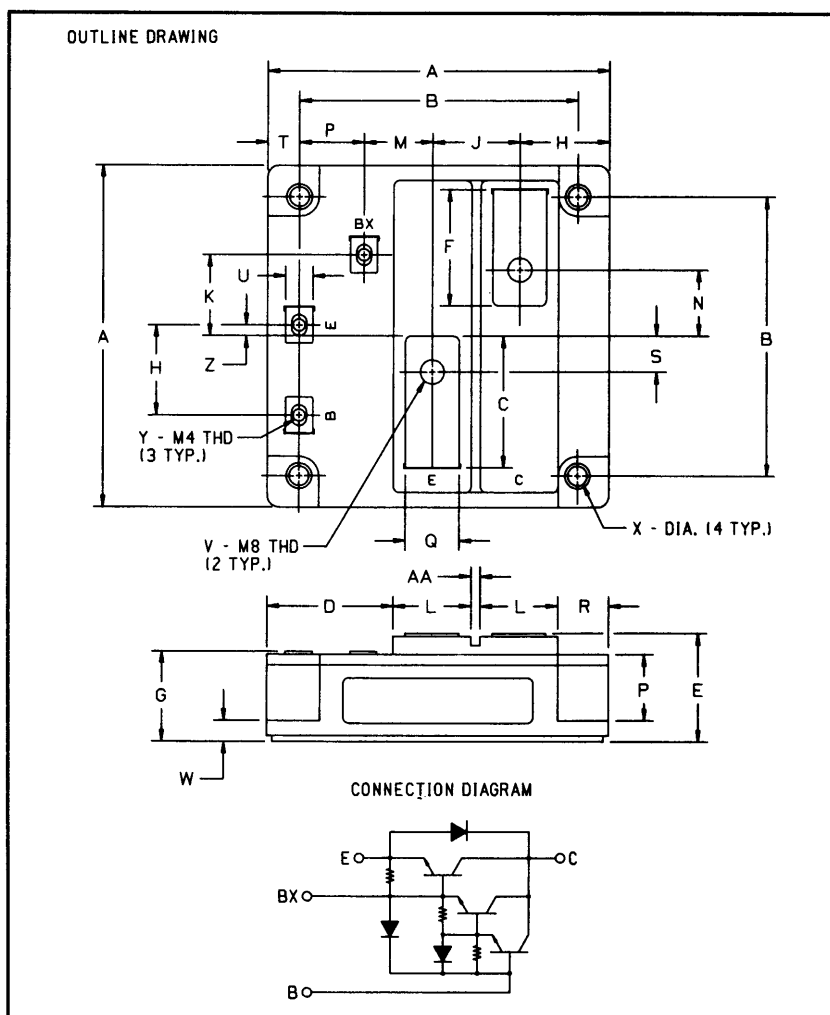
Outline Drawing
