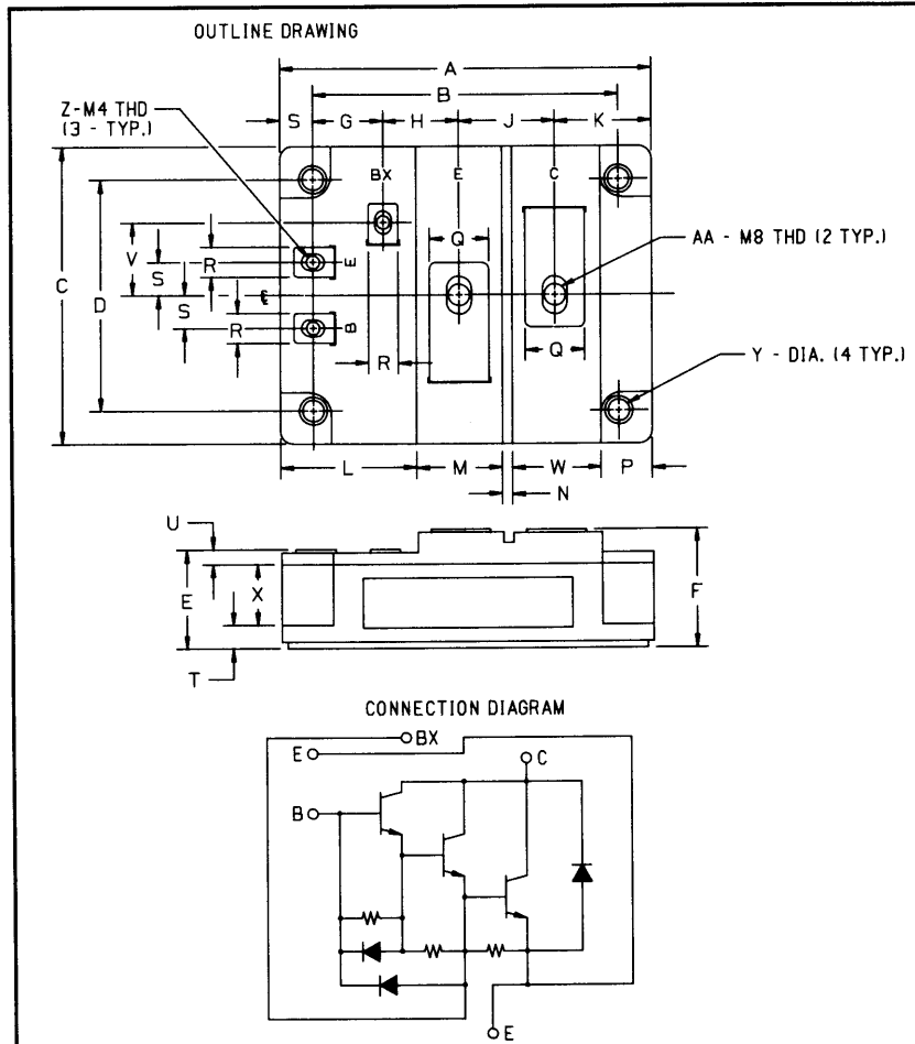
Outline Drawing
