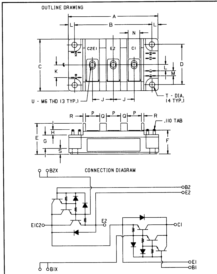
Outline Drawing
