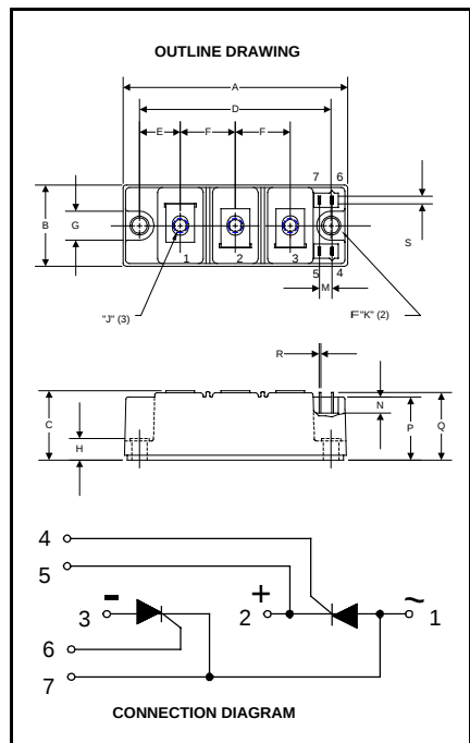
CD63__15A Dual SCR Isolated POW-R-BLOK™ Module Up to 160 Amperes & 1600 Volts
