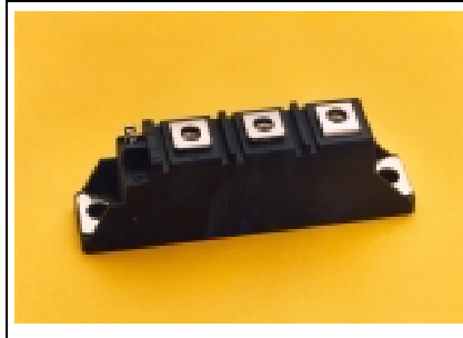
CD42__90, CD47__90 Dual SCR Isolated POW-R-BLOK™ Module 90 Amperes / Up to 1600 Volts
