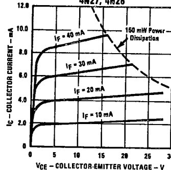
Collector Current vs Collector Emitter Voltage 4N27, 4N28
