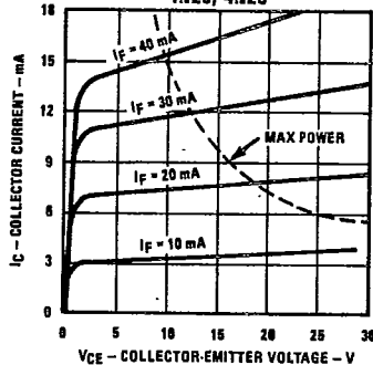
Collector Current vs Collector-Emitter Voltage 4N25, 4N26
