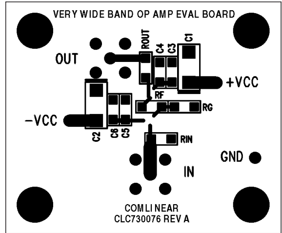
MSOP - Bottom Side
