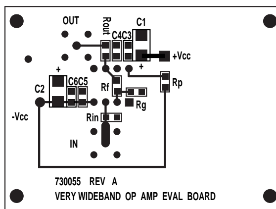
PDIP - Bottom Side
