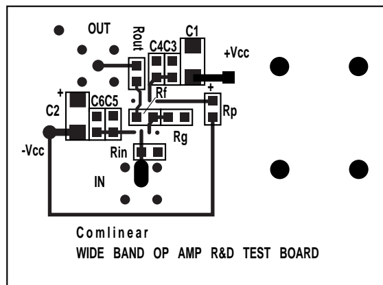
SOIC - Bottom Side
