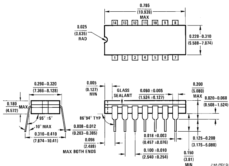
Cavity Dual-In-Line Package (J) Order Number MF6CJ-50 or MF6CJ-100 NS Package Number J14A
