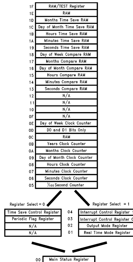
FIGURE 2. LV8573A Internal Memory Map
