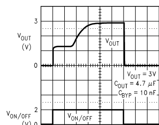
Turn-ON Waveform
