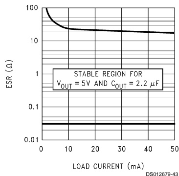
FIGURE 1. 5V/2.2 \mu\text{F} ESR Curves
