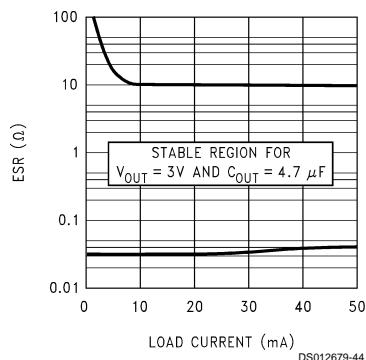
FIGURE 2. 3V/4.7 \mu\text{F} ESR Curves
