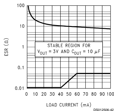
FIGURE 4. 3V/10 \mu F ESR Curves
