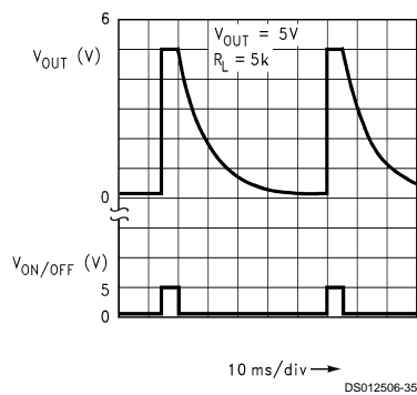
Turn-Off Waveform
