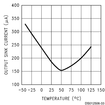
Output Reverse Leakage vs Temperature
