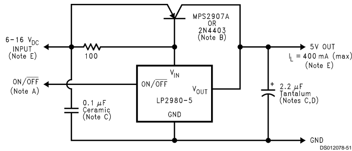
FIGURE 5. 5V/400mA Regulator
