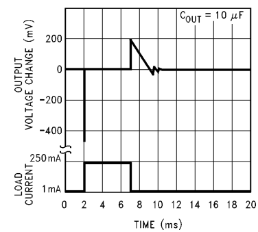
Load Transient
