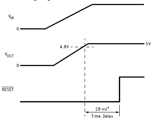
Timing Diagram for Timed Power-On Reset
