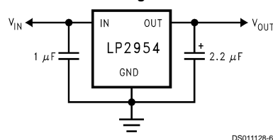
5V Regulator
