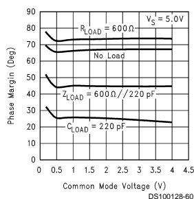
FIGURE 1. Phase Margin vs Common Mode Voltage for Various Loads
