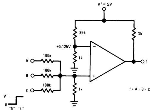
FIGURE 12. AND Gate
