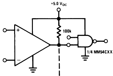
FIGURE 10. Driving CMOS
