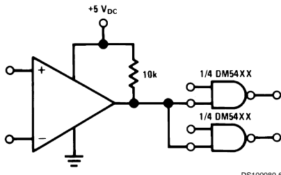
FIGURE 11. Driving TTL
