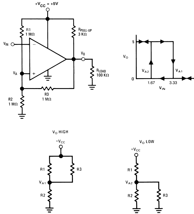
FIGURE 2. Inverting Comparator with Hysteresis
