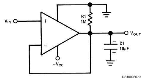
FIGURE 9. Negative Peak Detector
