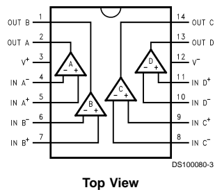
14-Pin SO/TSSOP
