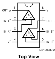
8-Pin SO/MSOP
