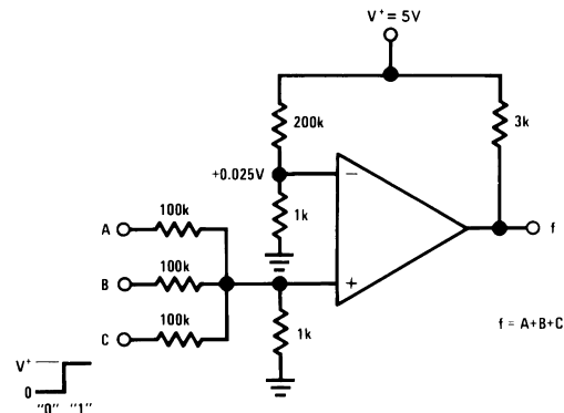
FIGURE 13. OR Gate
