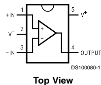
5-Pin SC70-5/SOT23-5
