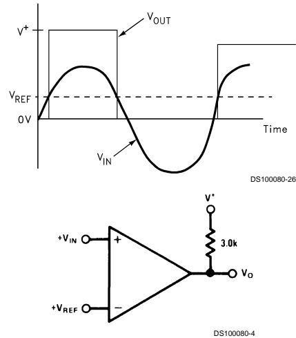
FIGURE 1. Basic Comparator
