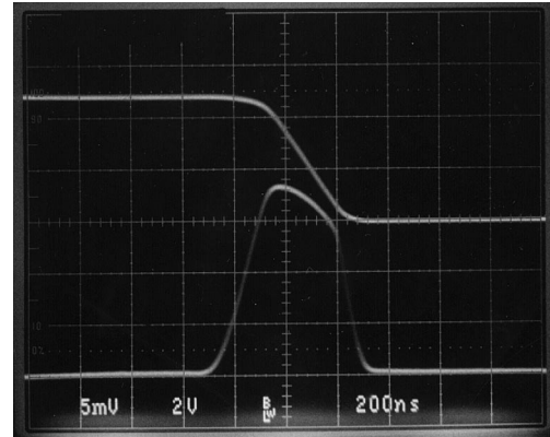
FIGURE 5. R_S = 10\Omega
