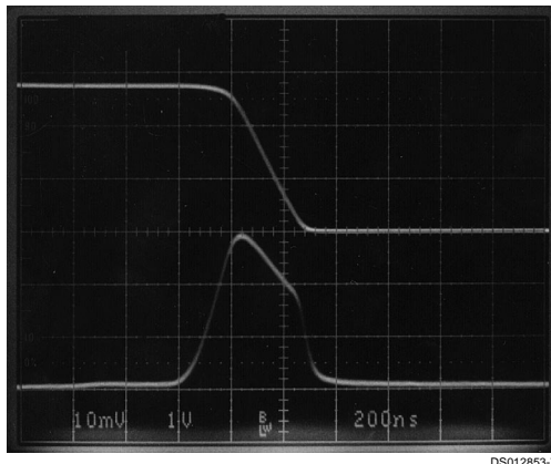
FIGURE 4. R_S = 100\Omega
