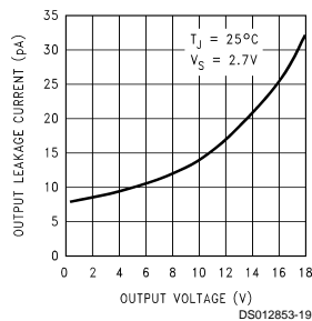
Output Leakage Current vs Output Voltage LMC7225
