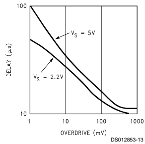
Prop Delay vs Overdrive
