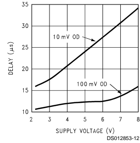
Prop Delay vs V_{\text{Supply}}
