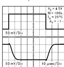
Inverting Small Signal Pulse Response at 10V
