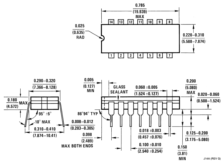
14-Lead Ceramic Dual-In-Line Pkg. (J) Order Number LMC660AMJ/883 NS Package Number J14A
