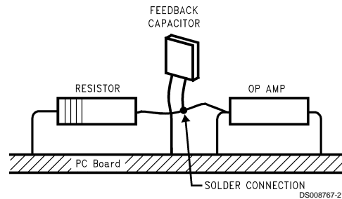
FIGURE 7. Air Wiring
