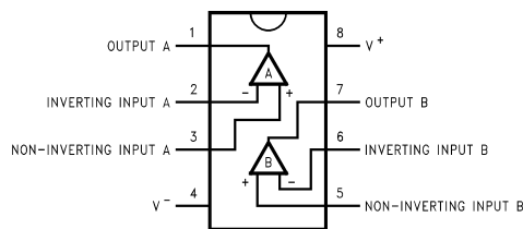
8-Pin DIP/SO/MSOP
