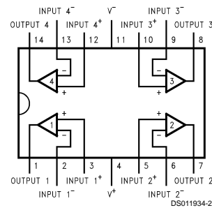
14-Pin DIP/SO
