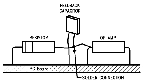
FIGURE 5. Air Wiring
