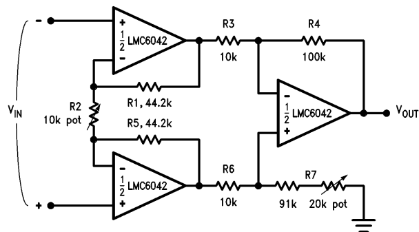
FIGURE 9. Instrumentation Amplifier
