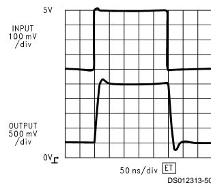
LM7131 Driving Flash A/D Load A_V = +5 @ +5V
