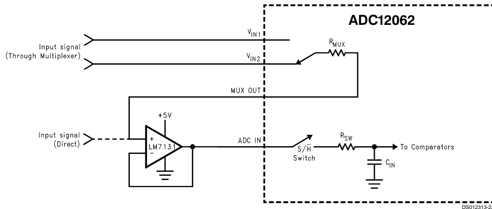
FIGURE 14. Buffering the Input with an LM7131 High Speed Op Amp
