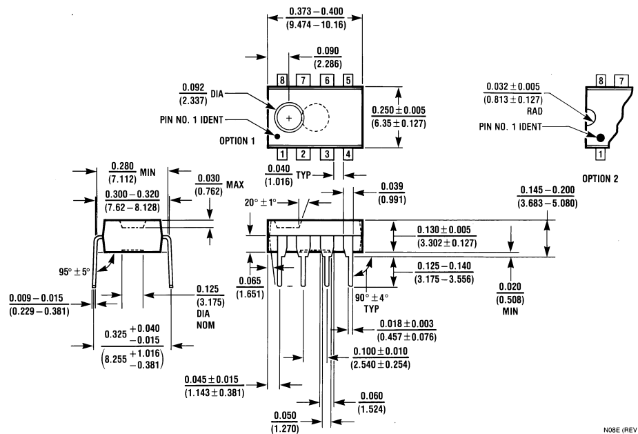
8-Pin Molded DIP 8-Lead (0.300" Wide) Molded Dual-In-Line Package Order Package Number LM7131ACN or LM7131BCN NS Package Number NO8E
