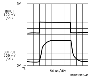
LM7131 Cable Driver A_V = +10 @ +3V
