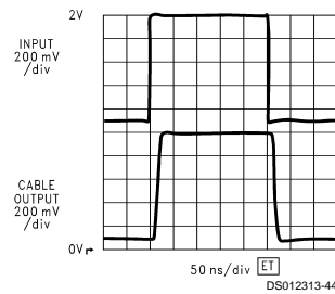
LM7131 Driving 5' RG-59 A_V = +2 @ +5V
