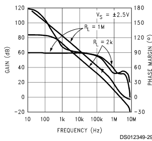
Gain and Phase vs Frequency
