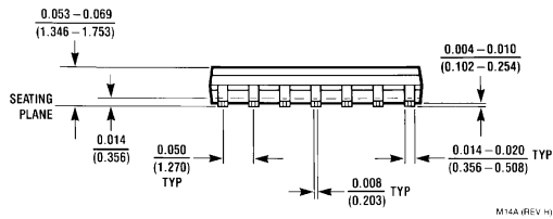
14-Lead (0.300" Wide) Molded Small Outline Package, JEDEC Order Number LM6134AIM, LM6134BIM, LM6134AIMX or LM6134BIMX NS Package Number M14A
