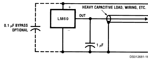
FIGURE 5. LM60 with Filter for Noisy Environment
