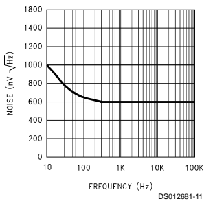
Noise Voltage
