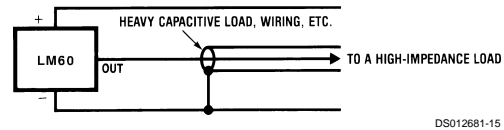
FIGURE 4. LM60 No Decoupling Required for Capacitive Load
