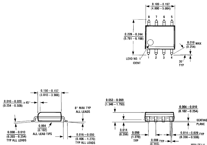
Order Number LM4881M NS Package Number M08A
