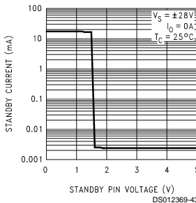
Standby Current ( I_{CC} ) vs Standby Pin Voltage
