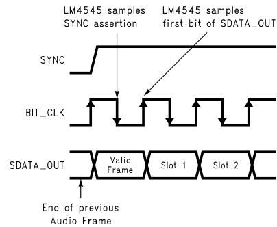
FIGURE 5. Start of Audio Output Frame
