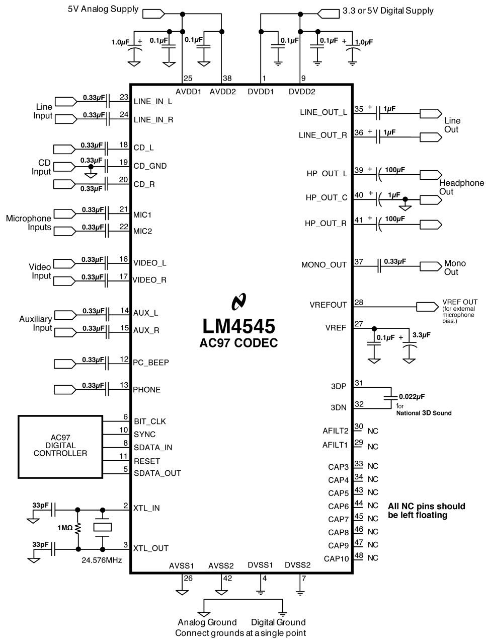
FIGURE 2. LM4545 Typical Application Circuit
