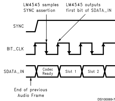
FIGURE 7. Start of Audio Input Frame
