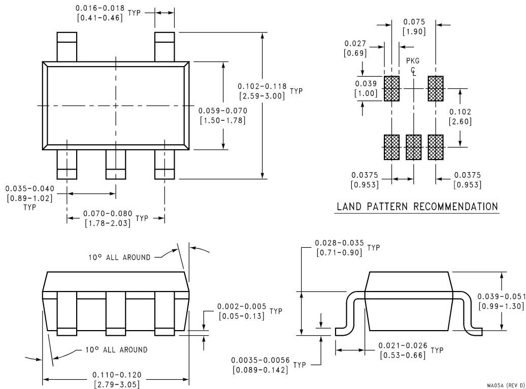
SOT-23 Package 5-Lead Small-Outline Package (M5) For Ordering, Refer to Ordering Information Table NS Package Number MA05A
