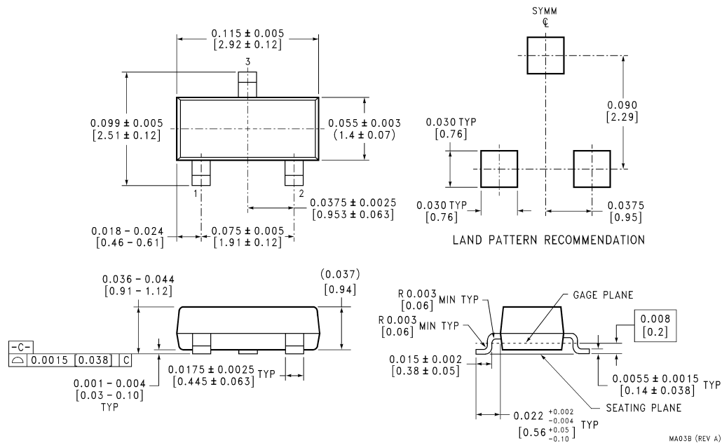
SOT-23 Package 3-Lead Small-Outline Package (M3) For Ordering, Refer to Ordering Information Table NS Package Number MA03B
