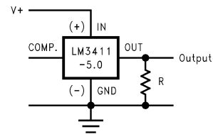
FIGURE 15. Voltage Detector
