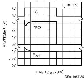
Response Time for 3.3V Version (Cc = 0 pF)
