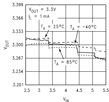
V_{OUT} vs. V_{IN}
