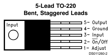
Front View Order Number LM2991T Flow LB03 See NS Package Number T05D
