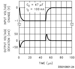
LM2990-12 and LM2990-15 Load Transient Response
