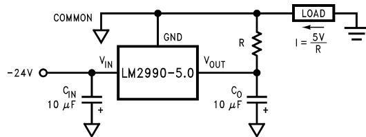
Fixed Current Sink
