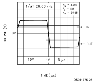
Pulse Response
