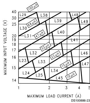
FIGURE 5. LM2678-12
