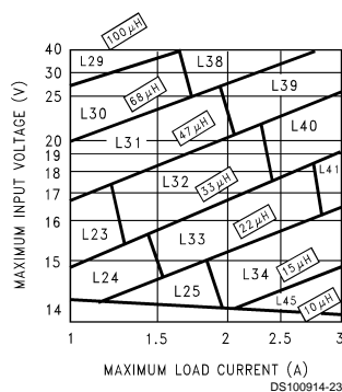
FIGURE 5. LM2676-12
