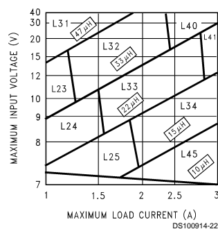
FIGURE 4. LM2676-5.0
