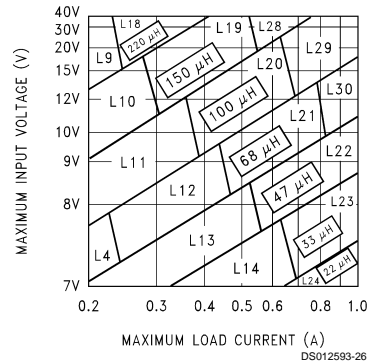
FIGURE 5. LM2598-5.0
