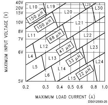
FIGURE 4. LM2598-3.3
