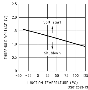
Shutdown/Soft-start Threshold Voltage
