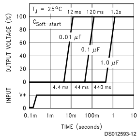
Soft-start Response
