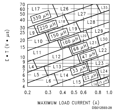
FIGURE 7. LM2598-ADJ
