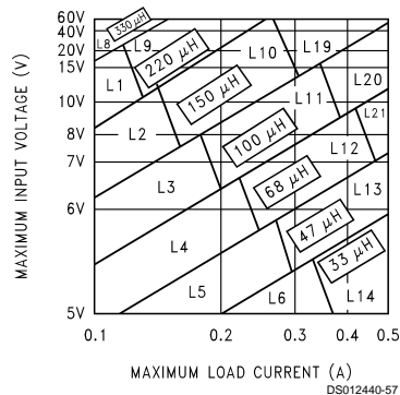
FIGURE 3. LM2597/LM2597HV-3.3
