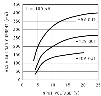
FIGURE 29. Maximum Load Current for Inverting Regulator Circuit
