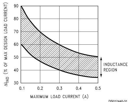
FIGURE 18. ( \Delta I_{L} ) Peak-to-Peak Inductor Ripple Current (as a Percentage of the Load Current) vs Load Current
