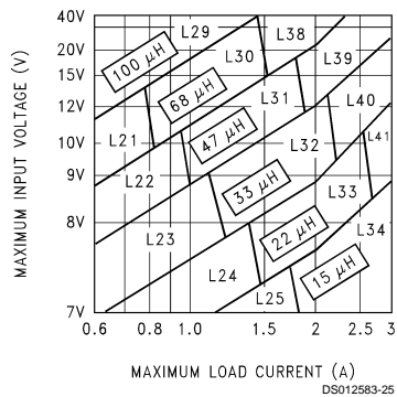
FIGURE 5. LM2596-5.0
