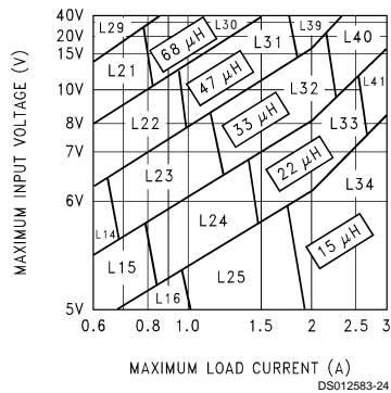
FIGURE 4. LM2596-3.3
