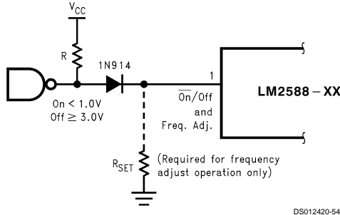
FIGURE 41. Shutdown Operation
