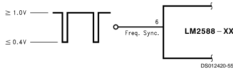
FIGURE 43. Frequency Synchronization
