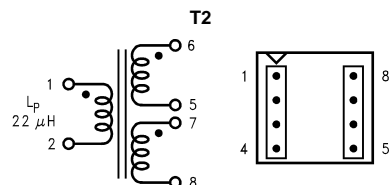
FIGURE 16. Coilcraft Q4337-B
