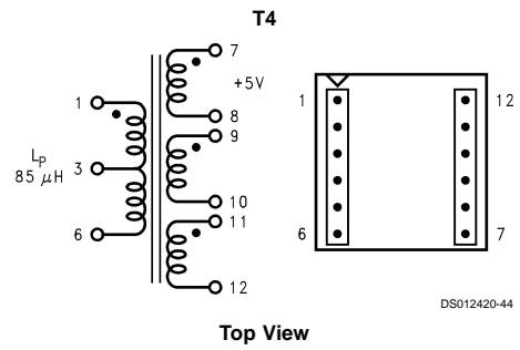
Top View FIGURE 28. Renco RL-5535
