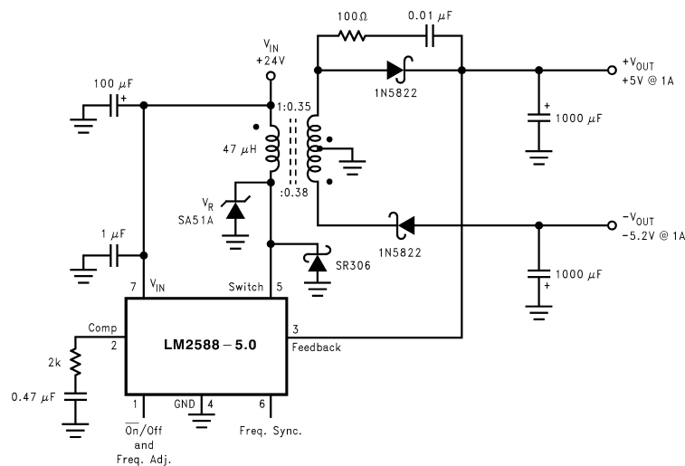
FIGURE 46. Flyback Regulator
