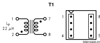
FIGURE 15. Coilcraft Q4434-B
