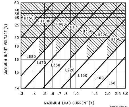
FIGURE 5. LM2576(HV)-12
