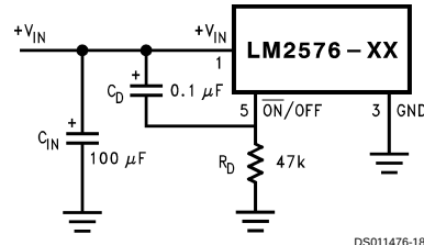
FIGURE 14. Delayed Startup
