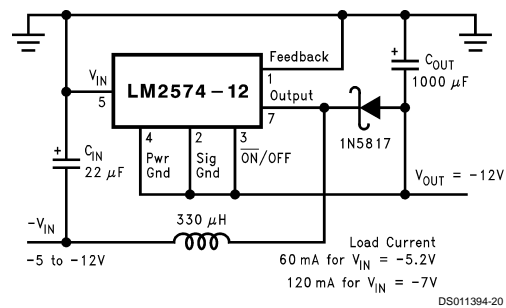
FIGURE 12. Negative Boost
